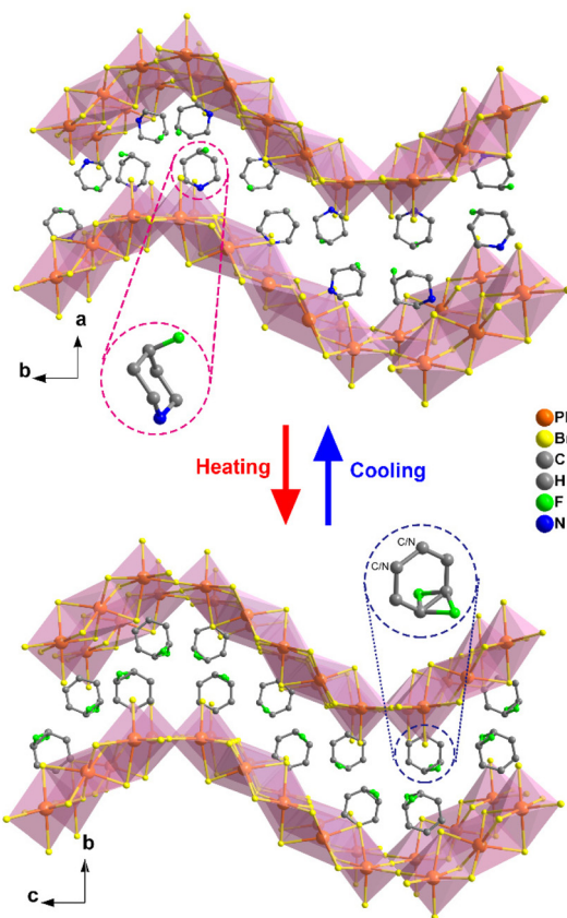
Fig. 2 Comparison of the packing structures of [\text{4-FPD}]_6\text{Pb}_5\text{Br}_{16} at 299 K (upper) and 440 K (lower). All the hydrogen atoms were omitted for clarity.
