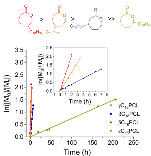
Fig. 4 Semi-logarithmic kinetic plot for ROP of \epsilon\text{C}_{18}\text{CL} , \gamma\text{C}_{18}\text{CL} and \beta/\delta\text{C}_{18}\text{CL} isomers using DPP (10 mol%) and 4-methoxybenzyl alcohol as initiator ( [\text{M}]_0/[\text{I}]_0 = 50 ). \ln([\text{M}]_0/[\text{M}]_t) was determined by ^1\text{H} NMR spectroscopy.
