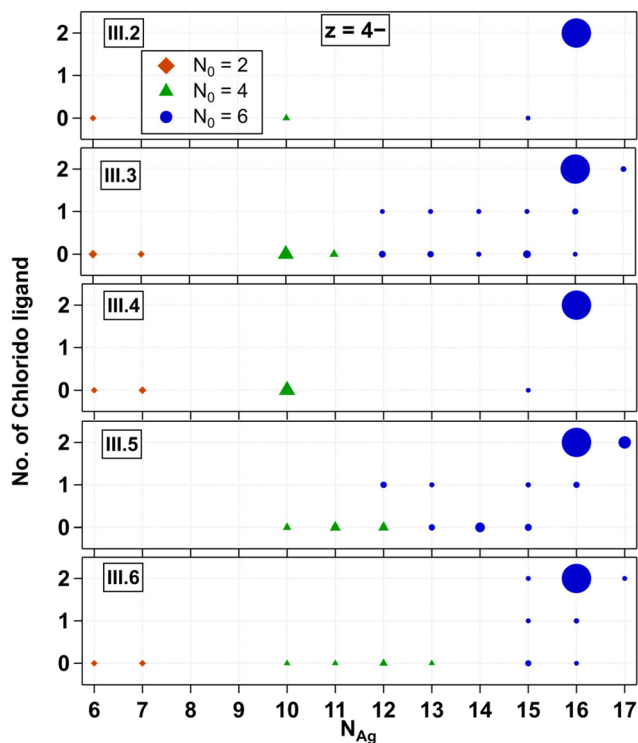
Fig. 4 N_0 and N_{\text{Ag}} of mass peaks of Group III \text{Ag}_N -DNAs for charge state z = -4 . Number of chlorido ligands is represented on the vertical axis. All species are stabilized by n_s = 2 DNA oligomers. N_0 = 6, 4 , and 2 are denoted by blue circles, green triangles, and ochre diamonds, respectively.
