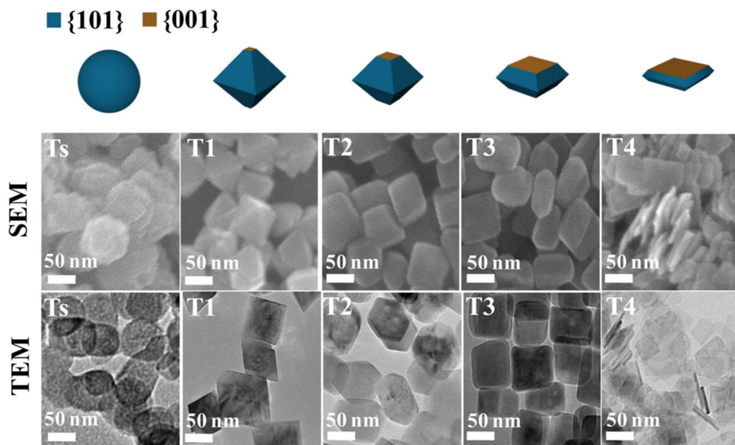
Fig. 4 SEM and TEM images of the \text{TiO}_2 nanocrystals with different degrees of the \{001\} facet synthesized at various ratios of HF/ \text{H}_2\text{O} . Reprinted with permission from ref. 63. Copyright 2017, American Chemical Society.
