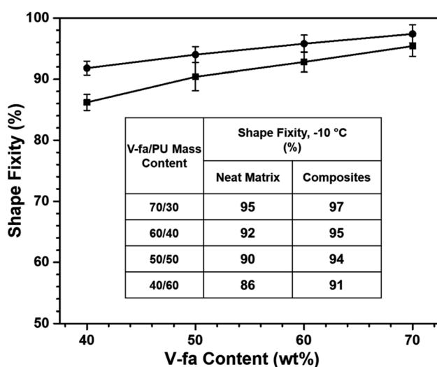
Fig. 6 Shape fixity value of (■) neat poly(V-fa/urethane) and (●) poly(V-fa/urethane) nanocomposites filled with 3 wt% GNPs.
