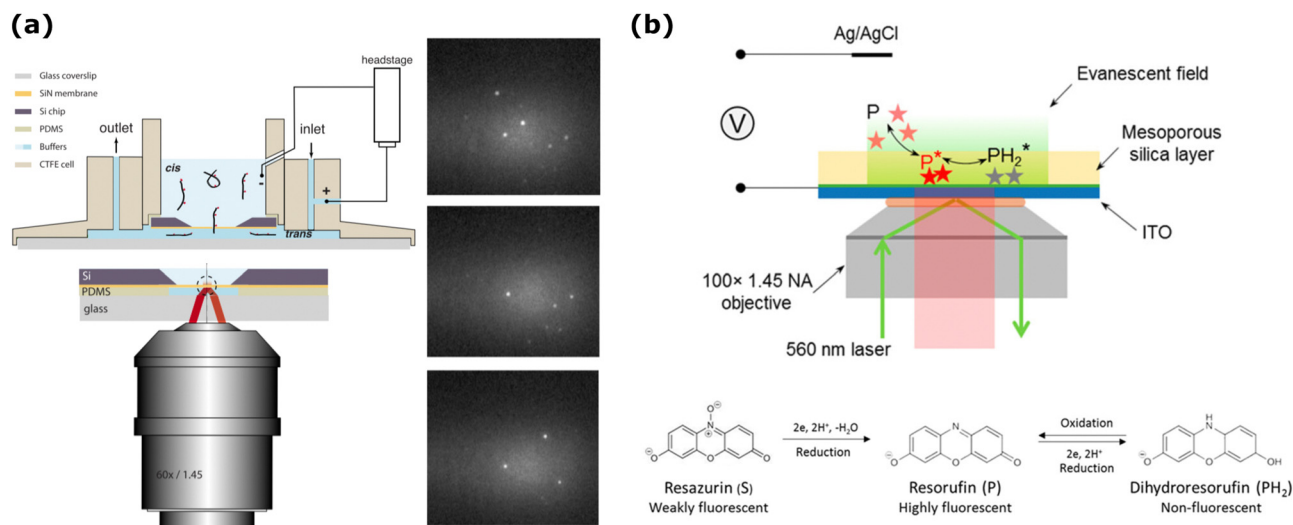
Fig. 7 (a) (Right) The cartoon on the left presents the TIRF method used to investigate single-molecule detection from 1D thin \text{SiN}_x nanoporous film (orange color) sandwiched between two aqueous fluids. Schematic illustration on the left-top presents the flow cell setup to mobilize the ATTO647N fluorophore conjugated DNA molecules towards the nanopores by the applied voltage and image them at this nanoconfinement. (Right) Images of the \text{SiN} membrane where individual DNA molecules were trapped. Reprinted from ref. 274 with the permission of AIP Publishing. (b) (Top) Scheme presenting the setup used for single-molecule electrochemistry detection from a porous 1D nanoporous silica-coated ITO electrode. (Bottom) Irreversible reduction of Resazurin (weakly fluorescent) to Resorufin (highly fluorescent) and the redox reaction between resorufin and Dihydroresorufin (non-fluorescent), which is reversible. Reprinted with permission from ref. 277 Copyright 2017, American Chemical Society.
