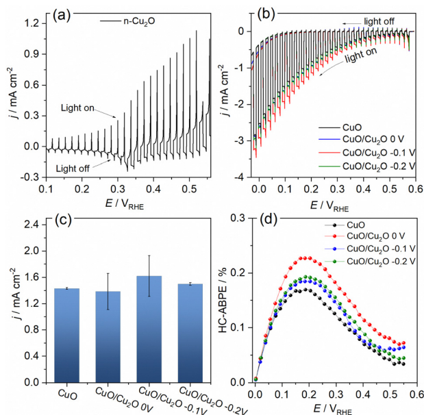
Fig. 4 Linear sweep voltammograms at 5 \text{ mV s}^{-1} under 1.5G pulsed illumination ( 100 \text{ mW cm}^{-2} ) of (a) Cu 2 O and (b) CuO, CuO/Cu 2 O 0 V, CuO/Cu 2 O –0.1 V and CuO/Cu 2 O –0.2 V in 0.5 \text{ mol L}^{-1} Na 2 SO 4 solution (pH 6). (c) Mean and standard deviation of the photocurrent density values obtained at 0.1 \text{ V}_{\text{RHE}} . (d) HC-ABPE efficiency for CuO and CuO/Cu 2 O films.
