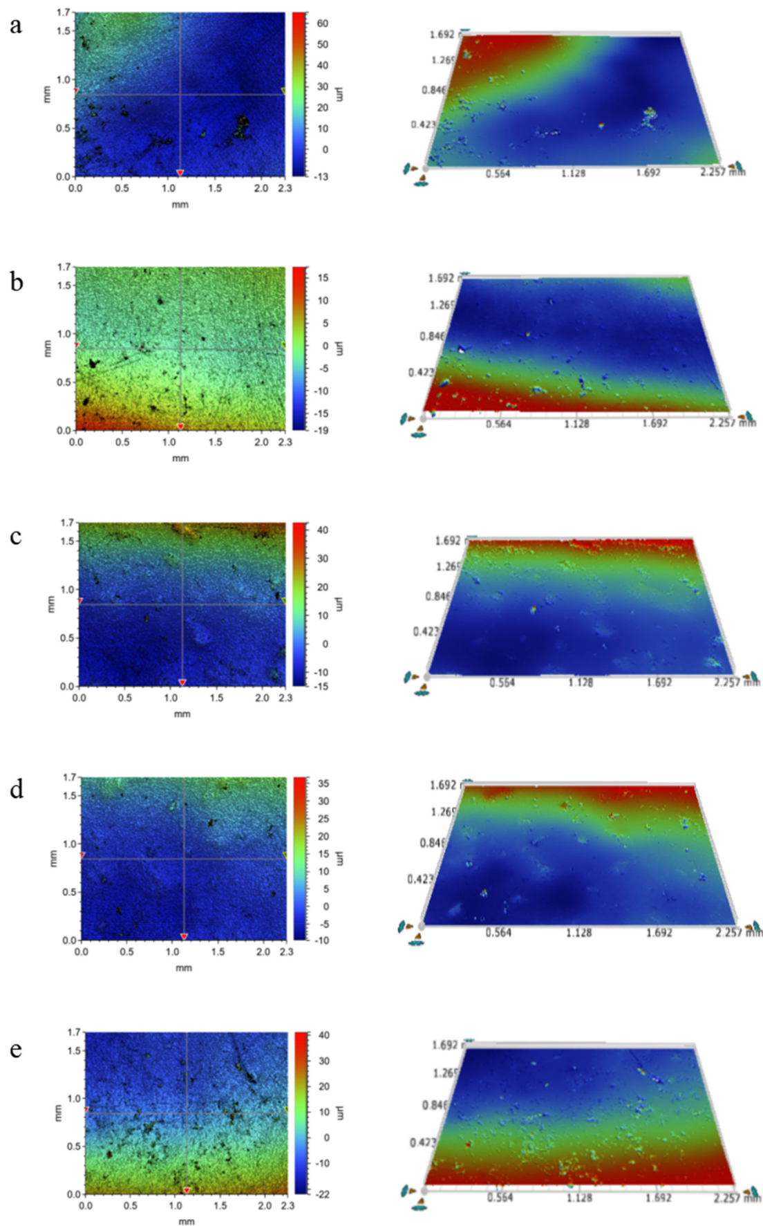
Fig. 7 (a-e) Surface morphology (left) of a pure PE sample soaked in oilfield water for 10, 17, 24, 31 and 38 days, respectively, and the 3D topography (right) after flattening.
