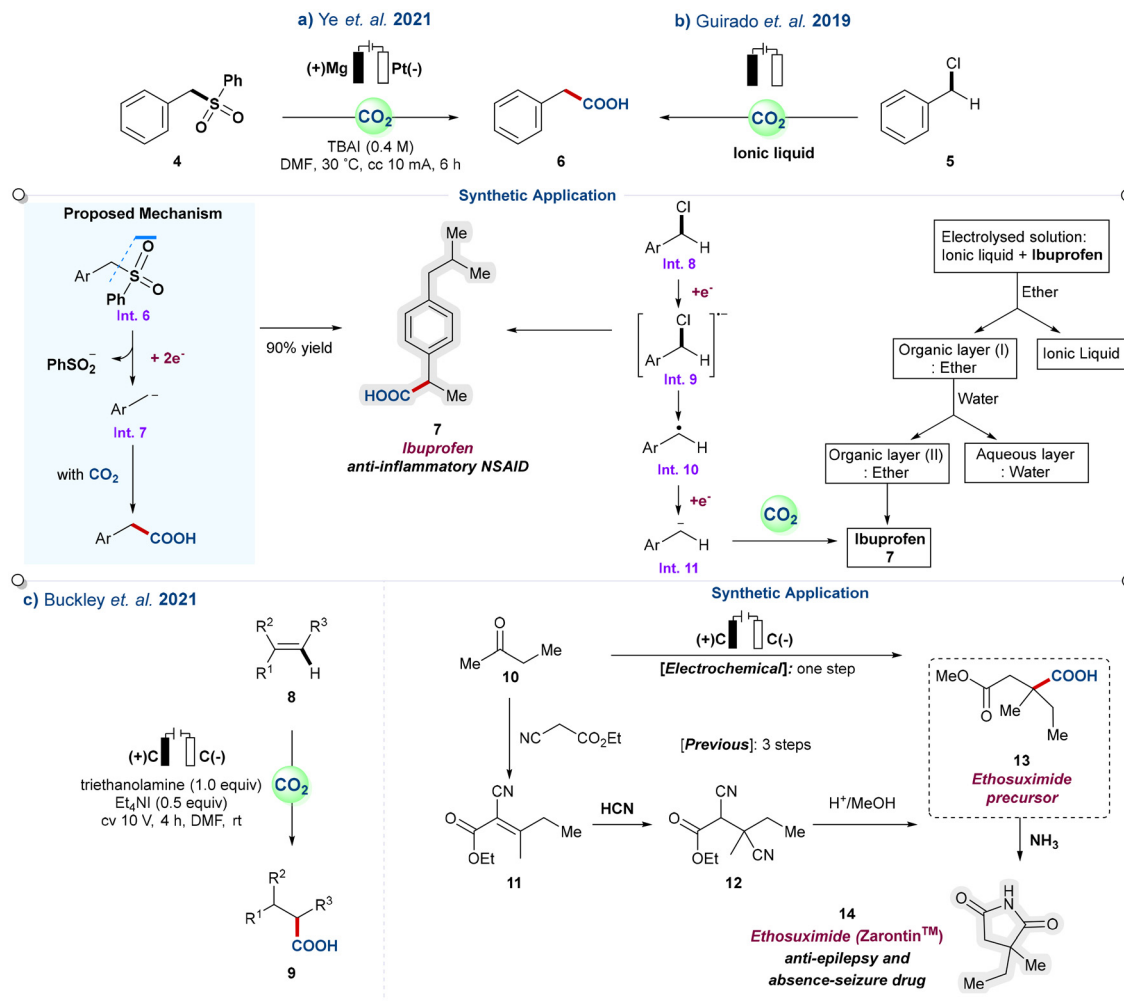
Scheme 2 (a) Desulfonylative electrocarboxylation of sulfones for the synthesis of Ibuprofen (ref. 25). (b) Electrocarboxylation of benzyl halides in ionic liquids (ref. 26). (c) Selective electrosynthetic hydrocarboxylation of \alpha,\beta unsaturated esters (ref. 27).
