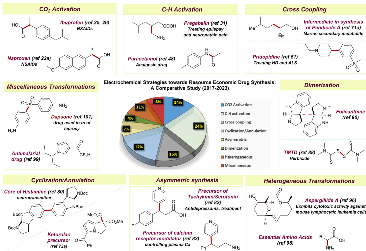
Fig. 1 Representative examples of drug molecules synthesised using electrocatalytic approaches.
