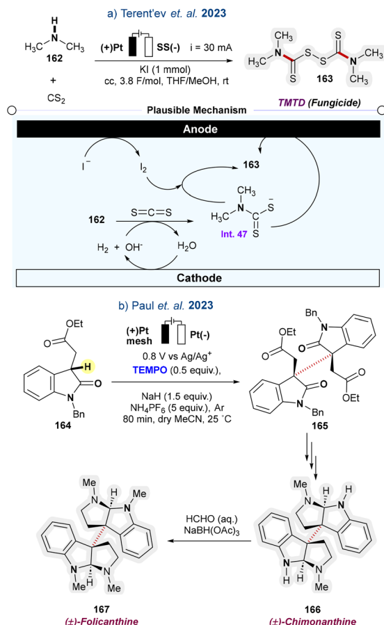
Scheme 22 (a) Electrochemical dimerisation for the synthesis of fungicides (ref. 88). (b) Electrochemical dimerisation of 3-substituted-2-oxindoles for the syntheses of folicanthine and chimonanthine (ref. 90).
