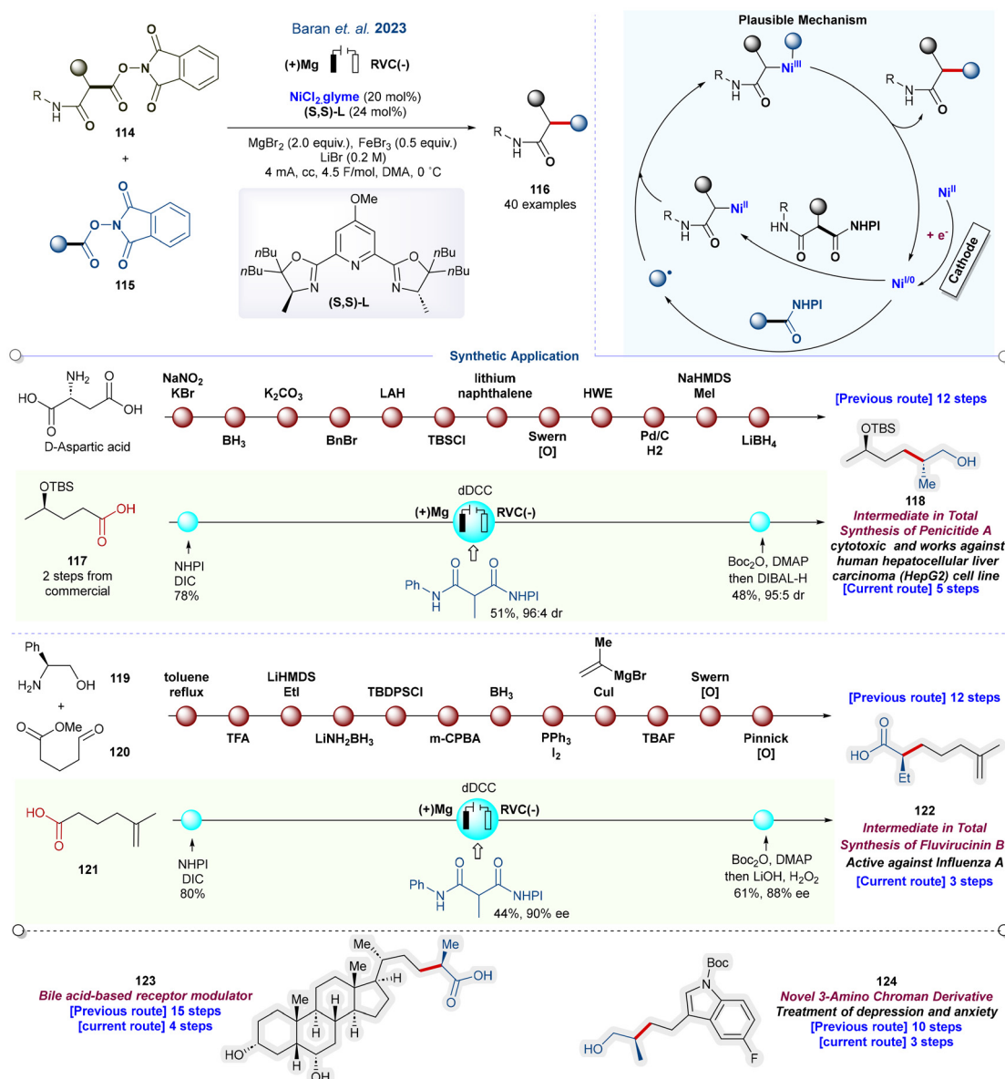
Scheme 15 Enantioselective doubly decarboxylative \text{C}(\text{sp}^3)\text{--}\text{C}(\text{sp}^3) cross coupling (ref. 71a).
