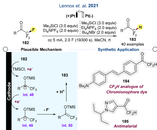
Scheme 24 Electrochemical hydrodefluorination to difluoromethyl ketones (ref. 99).
