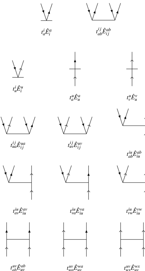
Fig. 1 Goldstone diagrams for the singles and doubles amplitudes used in our NOECCSD. Core and virtual electrons are represented by solid arrows; active electrons are represented by skeleton arrows.
