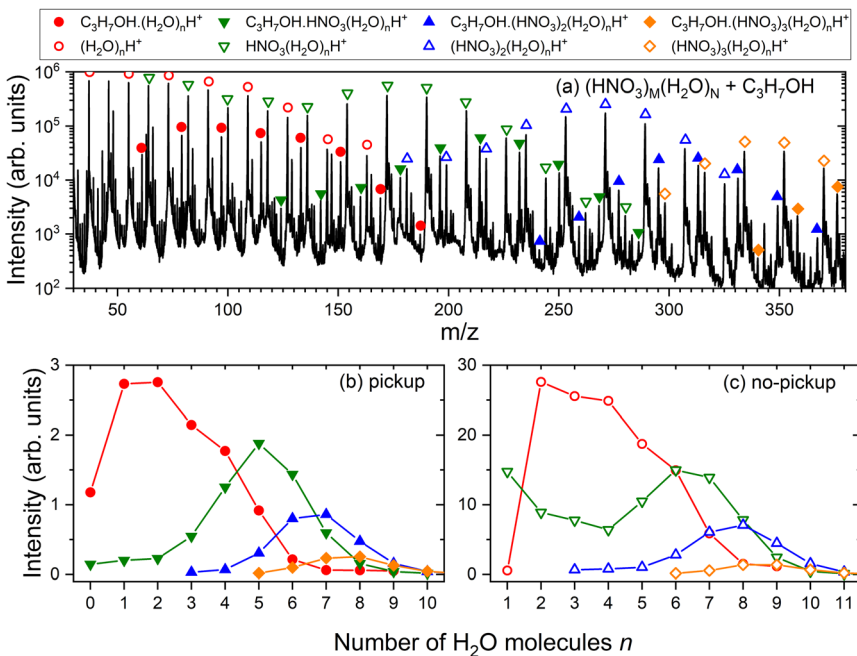
Fig. 3 (a) The mass spectrum of (HNO_3)_M(H_2O)_N clusters after the uptake of 1-propanol. The open symbols denote the (HNO_3)_m(H_2O)_n H^+ series and the full symbols denote the C_3H_7OH \cdot (HNO_3)_m(H_2O)_n H^+ ions. (b) Integrated intensities of the C_3H_7OH \cdot (HNO_3)_m(H_2O)_n H^+ mass peaks as a function of the number of water molecules n . (c) The same for the (HNO_3)_m(H_2O)_n H^+ mass peaks.
