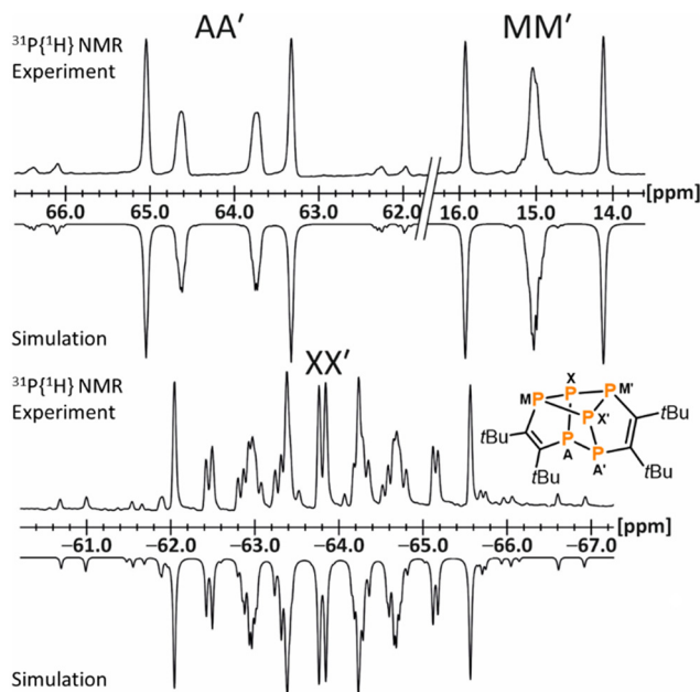
Fig. 6 Sections of the 31 P{ 1 H} NMR spectrum of 13 with nuclei assigned to an AA'MM'XX' spin system; experimental (top); simulation (bottom): \delta(P_{AA'}) = 64.2 ppm, \delta(P_{MM'}) = 15.0 ppm, \delta(P_{XX'}) = -63.8 ppm, ^1J_{AA'} = -261.9 Hz, ^1J_{AX'} = ^1J_{A'X'} = -293.9 Hz, ^1J_{M'X'} = ^1J_{MX'} = -134.2 Hz, ^2J_{AM} = ^2J_{A'M'} = -3.2 Hz, ^2J_{A'M} = ^2J_{AM'} = 9.9 Hz, ^2J_{MM'} = 24.9 Hz, ^2J_{AX'} = ^2J_{A'X'} = 15.3 Hz, ^1J_{MX} = ^1J_{M'X'} = -157.7 Hz, ^2J_{XX'} = 29.5 Hz.
