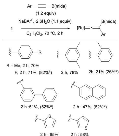
Fig. 10 Substrate scope ( [\text{Ru}] = [\text{Ru}(\text{dppe})\text{Cp}]^+ ).
