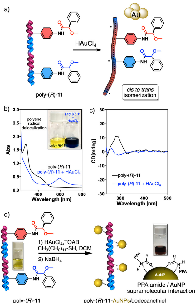
Fig. 48 (a) Schematic representation for the formation of radicals in poly-( R )-11 in presence of HAuCl 4 . (b) UV-vis and (c) CD spectra of poly-( R )-11 and poly-( R )-11 in presence of HAuCl 4 . (d) Schematic representation for the formation of poly-( R )-11-AuNPs nanocomposites by a variation of Brust–Schiffrin method. Reproduced from ref. 247 with permission from John Wiley and Sons, copyright 2021.
