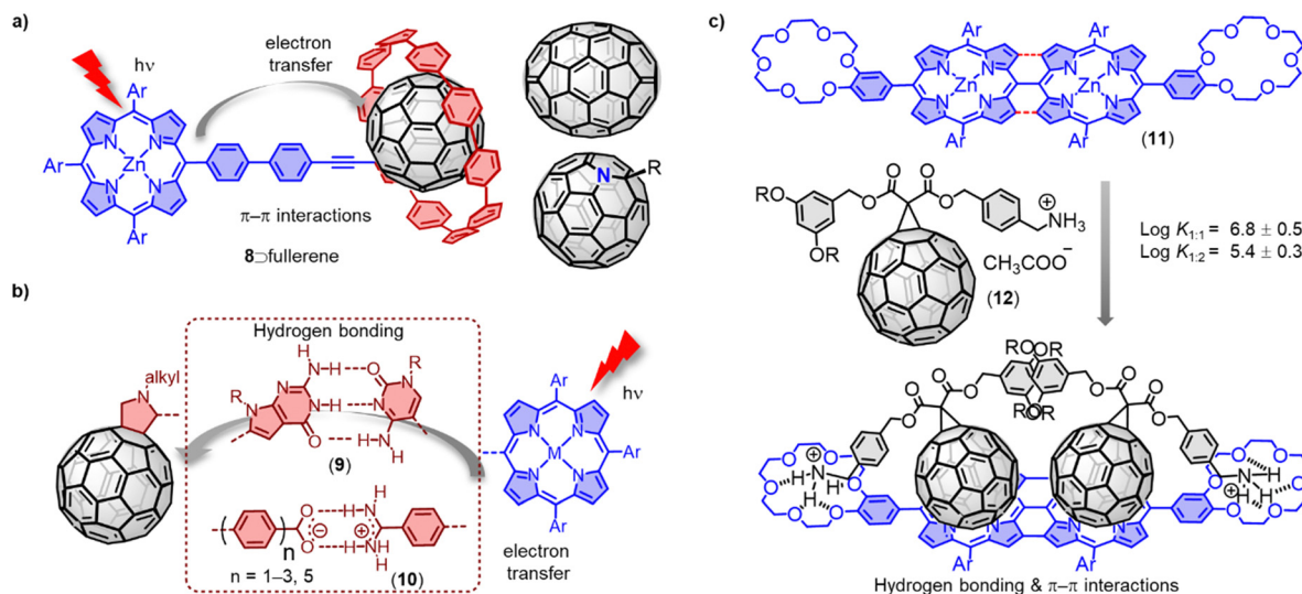
Fig. 7 (a) Efficient electron transfer in modular 8 fullerene complexes. (b) Selected examples of hydrogen bond bridged C_{60} -based D–A dyads ( 9 and 10 ) and corresponding charge transfer process. (c) Supramolecular complexation between ditopic porphyrin receptor 11 and fullerene derivative 12 .
