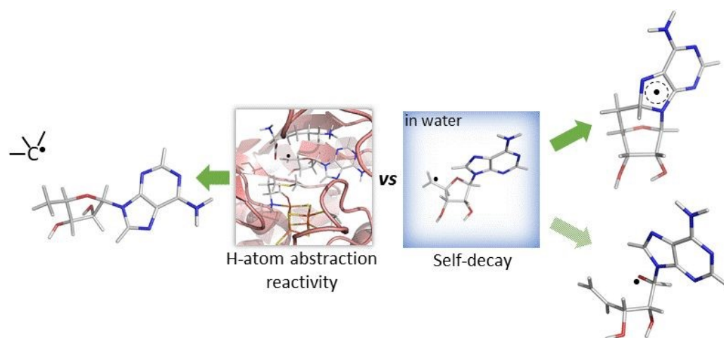
Scheme 2. Reactivity of the 5'-deoxyadenosyl radical in water vs. enzymatic environment. While 5'dAdo • is well known to be competent as an H-atom abstractor in radical SAM enzymes (the left side of the scheme), 17,18 it is unstable in water, undergoing an experimentally documented pathway – cyclization 20 (the product of which is shown in the right upper corner of the scheme) and a self-decay pathway as suggested by this computational work, yielding two fragments via ribosyl-ring opened intermediate 21 depicted in the right lower corner of the scheme.
