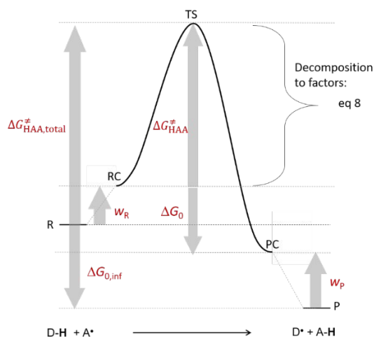
Scheme 3. The key energetics for bimolecular HAA reaction.
