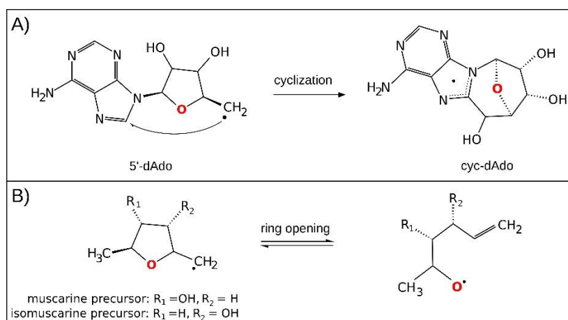
Figure 1. A. In the cyclization decay mechanism, the 5'dAdo • radical undergoes intramolecular radical addition leading to a stable cyclic structure. 20 B. The ring-opening decay mechanism was observed for the radicals similar to 5'dAdo • . 21
