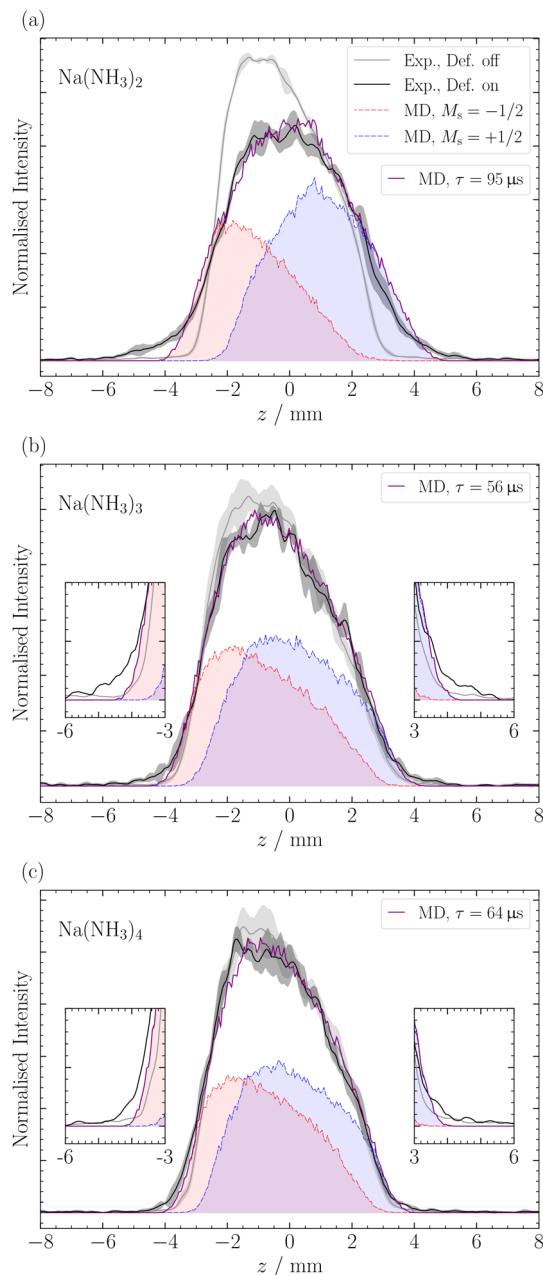
Fig. 6 Magnetic deflection of \text{NaNH}_3)_n , 2 \leq n \leq 4 ((a)–(c)), measured at M_r = 1 and at a current of 700 A. The grey and black error bars correspond to the experimental spatial distributions when the deflector is off and on, respectively. The purple line illustrates the total deflection observed in our simulations, while the red and blue shaded areas delineate the contributions of the two spin projections. Notably, for clusters larger than \text{NaNH}_3)_1 , the deflection deviates from that expected for a spin-1/2 system. The figure showcases the deflection with the \chi^2 -optimized \tau values. Shaded areas represent uncertainties at 1\sigma .
