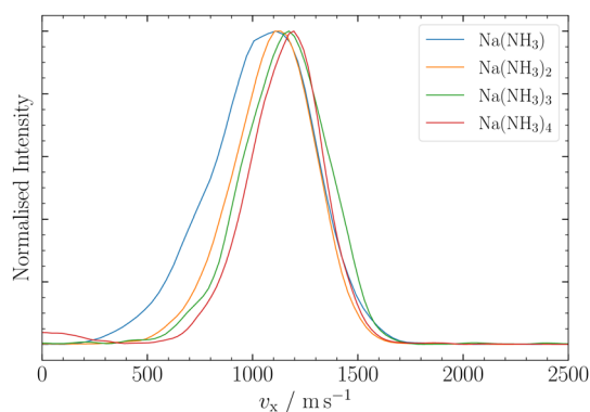
Fig. 5 Ion VMI results for \text{NaNH}_3)_n , n = 1-4 . \text{NaNH}_3)_1 and \text{NaNH}_3)_2 were measured with a nozzle temperature of T = 25 \text{ }^\circ\text{C} , whereas \text{NaNH}_3)_3 and \text{NaNH}_3)_4 were measured at T = 100 \text{ }^\circ\text{C} .
