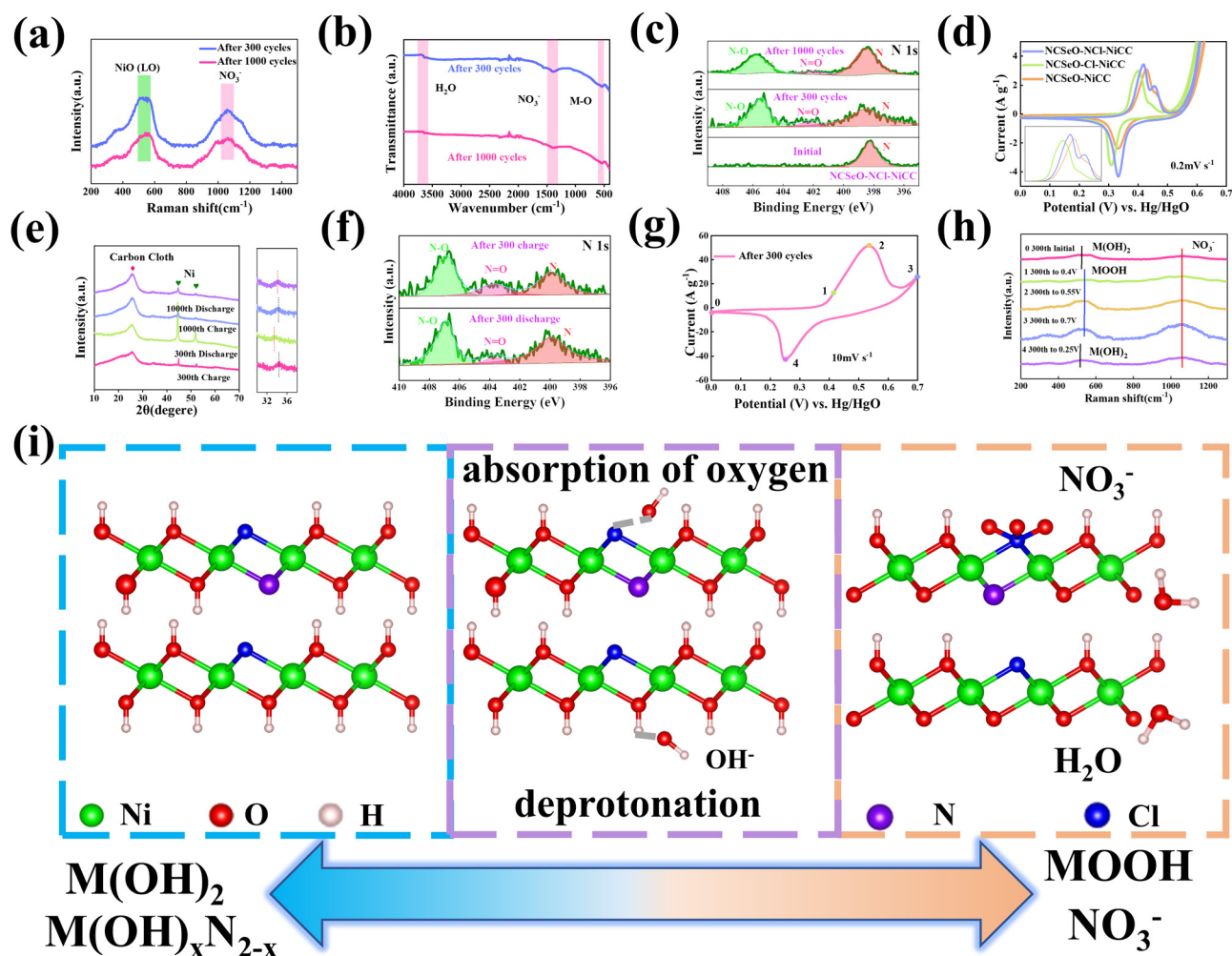
Fig. 5 (a) Raman spectra and (b) FTIR of NCSeO-NCl-NiCC after 300 cycles. (c) N 1s XPS spectra of NCSeO-NCl-NiCC for different cycles. (d) CV curves of various electrodes at a scan rate of 0.2 mV s -1 . (e) Ex situ XRD patterns of NCSeO-NCl-NiCC after various cycles. (f) N 1s XPS spectra of NCSeO-NCl-NiCC at different states. (g) CV curves at a scan rate of 10 mV s -1 of NCSeO-NCl-NiCC after 300 cycles. (h) Ex situ Raman spectra of NCSeO-NCl-NiCC in an electrochemical process. (i) Schematic illustration of the energy storage mechanism of M(OH)_2 and M(OH)_xN_{2-x} .
