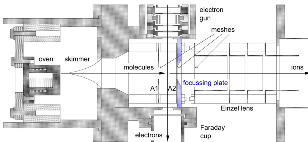
Fig. 1 Overview of the interaction region showing the oven containing pyrene, the skimmer, the electron gun, and the Einzel lens at the entrance to the reflectron time-of-flight mass spectrometer. The electron gun and the Faraday cup are only partially shown. The focussing plate has been added to enhance the collection of singly-charged ions from double ionisations (see discussion in the text).
