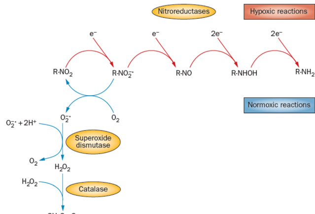
Fig. 7 Different radiation chemistry of nitro group under hypoxia and normoxia. While under normoxic conditions single electron reduction is in strong competition with the reduction of oxygen, under hypoxia multiple electron reduction occurs leading to a variety of reactive radical species. Reproduced from ref. 171 with permission from Springer Nature, copyright 2012.
