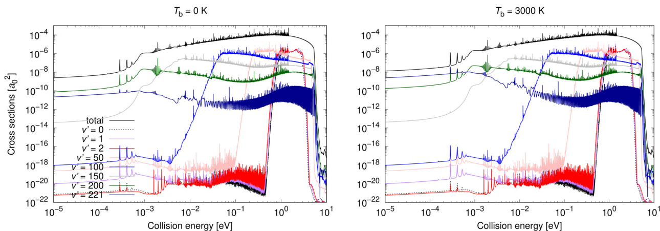
Fig. 4 Radiative association vibrationaly resolved cross sections obtained allowing for non-adiabatic dynamics for process (1) for two background temperatures: 0 K and 3000 K.
