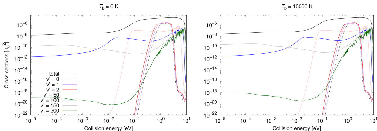
Fig. 5 Radiative association vibrationaly resolved cross sections for process (2) for two background temperatures, 0 K and 10 000 K.
