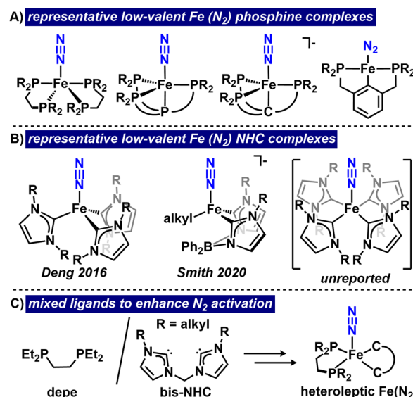
Fig. 1 (A) Fe phosphines demonstrated to activate N 2 . 2c,d,g,6a (B) Fe N 2 NHC complexes and the lack of a reported Fe N 2 tetracarbeno. 7b,c (C) Analogy between depe and bis-NHC ligand and the prospect of a heteroleptic complex.
