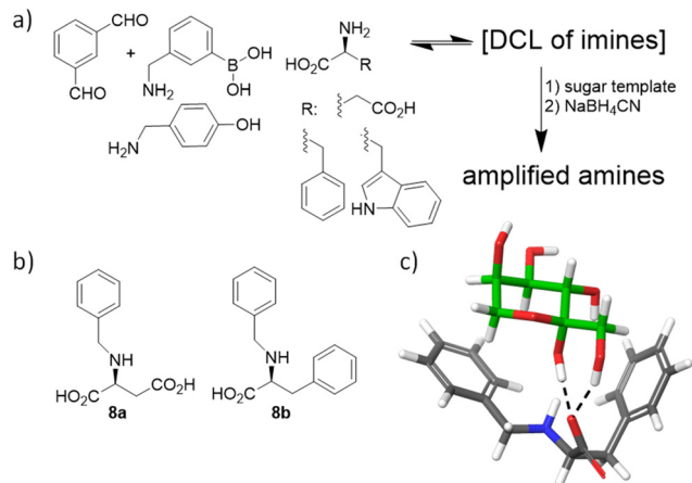
Fig. 7 (a) Sugar-templated DCL. (b) Simplified monosaccharide hosts thus identified. (c) Proposed model for the interaction of 8b with β-D-fructopyranose (green C-atoms).
