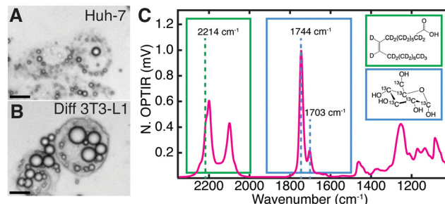
Fig. 2 Live cell characterization of the cell lines (A) Huh-7 and (B) differentiated 3T3-L1 after feeding with 2 H oleic acid (60 \mu M) and 13 C glucose (4.5 mg mL -1 ). Scale bars are 20 \mu m. (C) Full IR spectra of a point within a fixed Huh-7 cell LD 48 hours after feeding 2 H OA. 2 H-C from the 2 H oleic acid (green, structure in inset) which has been esterified in LDs. 2214 cm -1 is assigned to 2 H-C stretching. 13 C=O stretch at 1703 cm -1 where the 13 C comes from metabolized 13 C glucose (blue, structure in inset). Pictured alongside the unlabelled 12 C=O band at 1744 cm -1 .
