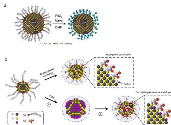
Fig. 11 (a) Lead halide exchange from an oleate capped PbS QCD to a halide-capped PbS QCD. Reprinted with permission from ref. 132. Copyright 2019, John Wiley & Sons, Inc. (b) Ligand exchange with lead halide anions and lead halide anions re-exchange with the functional ligands to render a p-type character process. Reprinted with permission from ref. 33. Copyright 2020, Springer Nature Limited.
