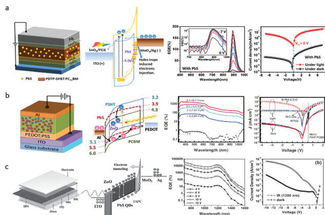
Fig. 10 (a) Device structure of the nanocomposite photodetectors; the energy diagram of the photodetectors under illumination without and with PbS QCD traps; EQE spectra with PbS QCDs, and dark current and photocurrent curves with PbS QCDs. Reprinted with permission from ref. 102. Copyright 2016, the Royal Society of Chemistry. (b) Device structure of the dual-quantum dot hybrid photodetector; the energy band diagram under illumination and reverse bias; EQE spectra of the device under reverse bias; photo- and dark-current density-voltage curves of P3HT:PCBM, PbS:P3HT:PCBM and PbS:P3HT:PCBM:ZnO devices. Reprinted with permission from ref. 103. Copyright 2014, John Wiley & Sons, Inc. (c) Device structure of a gain PbS QD photodiode; energy band diagram under illumination; EQE spectra as function of wavelength under different reverse bias; I - V curves under dark and under illumination intensities of 165\ \mu\text{W cm}^{-2} . Reprinted with permission from ref. 104. Copyright 2015, John Wiley & Sons, Inc.
