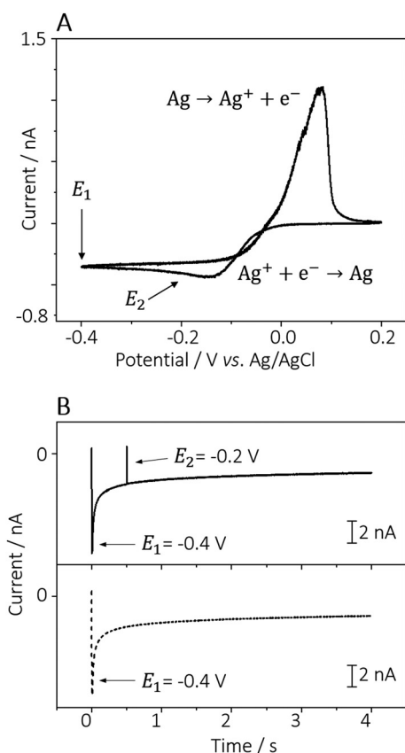
Fig. 1 (A) Cyclic voltammogram of a 0.5 mmol \text{L}^{-1} \text{AgNO}_3 in 50 mmol \text{L}^{-1} \text{KNO}_3 solution recorded at the PDA-modified gold electrode. The potentials applied for the electrodeposition of AgNPs ( E_1 and E_2 ) are highlighted with black arrows. (B) Exemplary current-time curves of the electrodeposition process via a double (continuous line) and single (dotted line) potentiostatic step. Conditions: \text{AgNO}_3 concentration: 0.5 mmol \text{L}^{-1} ; \text{KNO}_3 concentration: 50 mmol \text{L}^{-1} ; SECCM pipette diameter: 5 \mu\text{m} ; working electrode: PDA-modified gold electrode.
