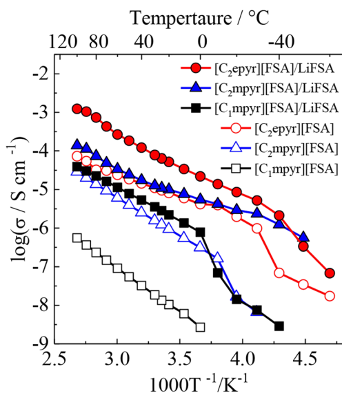
Fig. 3 Arrhenius plots of ionic conductivities for neat pyrrolidinium salts ( 1b ( [\text{C}_2\text{mpyr}][\text{FSA}] ), 2b ( [\text{C}_1\text{mpyr}][\text{FSA}] ), 3b ( [\text{C}_2\text{epyr}][\text{FSA}] )) and 5 mol% LiFSA-doped ones. Reprinted from ref. 43 with permission.
