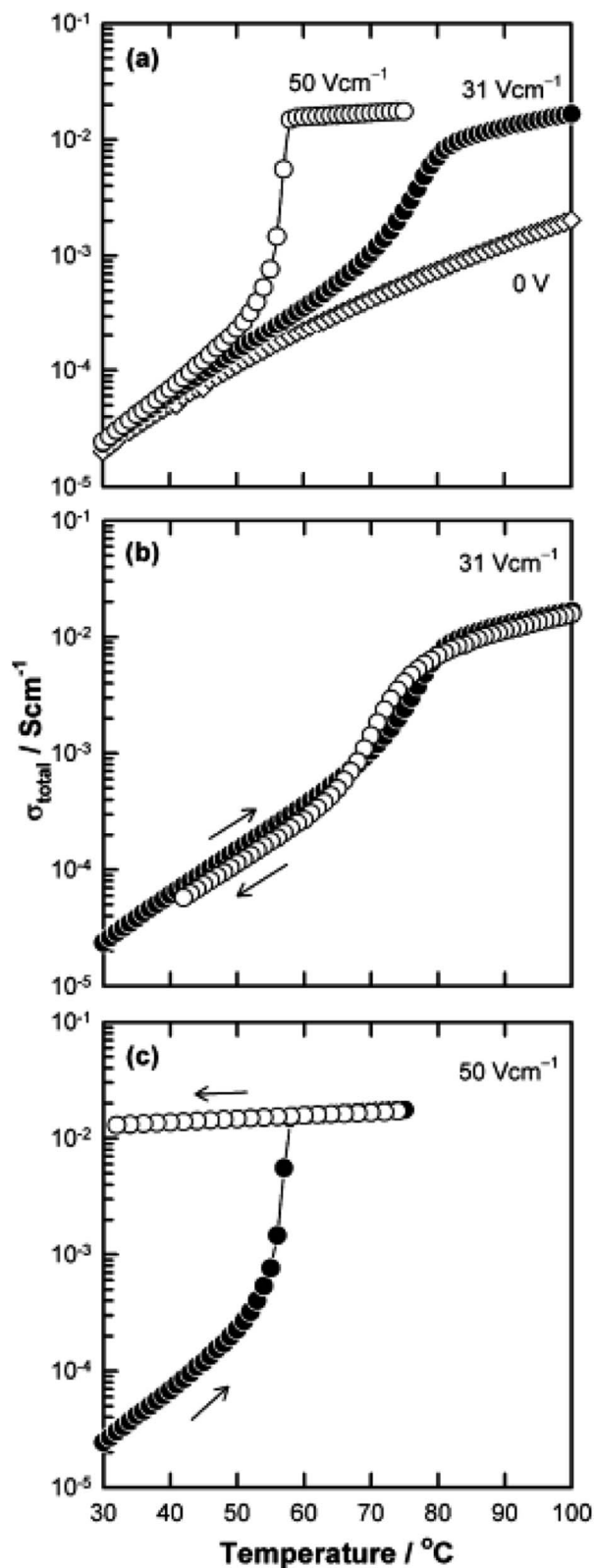
Fig. 7 Bulk conductivity of \text{Bi}_{0.95}\text{Ca}_{0.05}\text{FeO}_3 against temperature without and with applied fields of 31 and 50 \text{ V cm}^{-1} ; reproduced from N. Maso et al. , Phys. Chem. Chem. Phys. , 2014, 16 , 19408 with permission from the PCCP owner societies.
