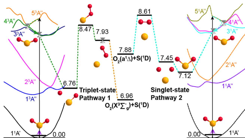
Fig. 4 Dissociation pathways of \text{SO}_2 leading to \text{O}_2(\text{X}^3\Sigma_g^-) + \text{S}^{\text{(1D)}} products via the triplet state manifold (left) and to \text{O}_2(\text{a}^1\Delta_g) + \text{S}^{\text{(1D)}} products via the singlet state manifold. The schematics of the simplified PECs for the ground and the first five excited states of ^3\text{A}'' symmetry (left) and the first five states of ^1\text{A}'' symmetry (right) support different paths leading to \text{S} + \text{O}_2 product formation. Dashed arrows indicate possible non-adiabatic pathways and the geometries and energies (in eV) of key intermediate structures along the dissociation pathways are also indicated. The horizontal axis represents the reaction coordinate, and the vertical axis is the potential energy (in eV).
