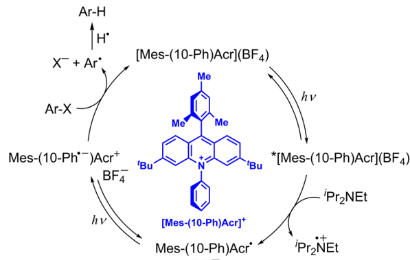
Scheme 4 Reductive dehydrogenation of aryl halide ( \text{Ar-X} ) with diisopropylamine by photoredox catalysis of [\text{Mes}-(10\text{-Ph})\text{Acr}](\text{BF}_4) . 37
