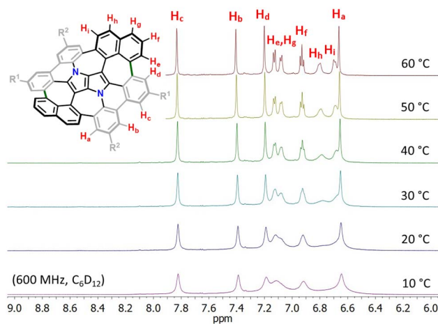
Fig. 3 Variable temperature ^1\text{H} -NMR spectrum of the molecular N-doped saddle 8 in the aromatic region (from 6.0 to 9.0 ppm) recorded in \text{cyclohexane-}d_{12} (600 MHz, 10–60 °C).
