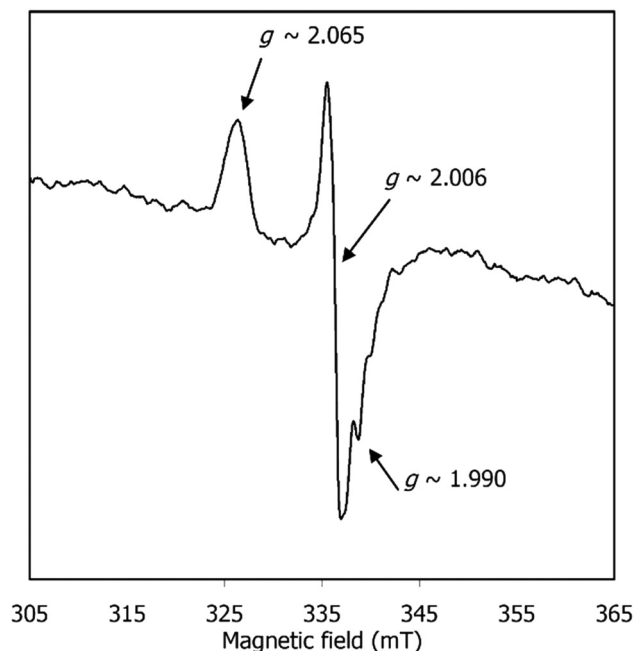
Fig. 8 EPR spectrum of [1] after CPE under CO 2 , in DMF at 90 K. Spectrum was acquired as described in the Experimental section.
