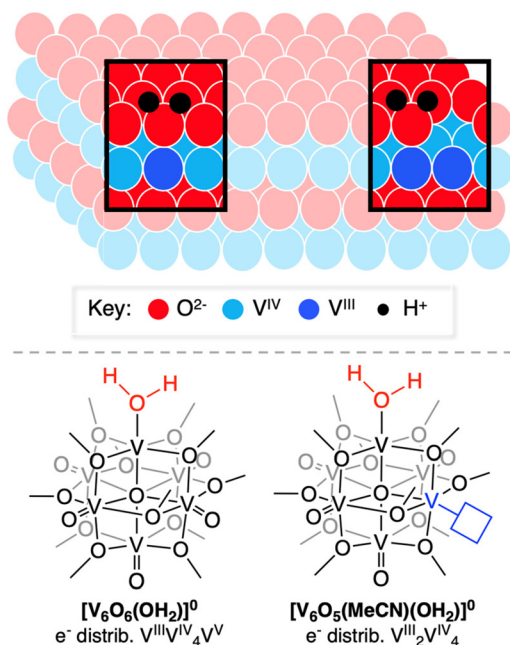
Fig. 1 PCET to the surface of pristine and O-deficient metal oxide surfaces (top). 2e - /2H + reduced POV-alkoxide clusters studied in this work, where V=O bond reduction occurs at the surface of a fully oxygenated vanadium oxide assembly, and one bearing a preformed O-atom vacancy to generate aquo-ligated cluster complexes.
