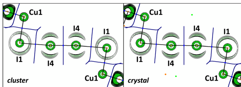
Fig. 8 OEP distribution in the plane of the polyiodide chain computed for cluster (left) and crystal (right) models of [\text{Cu}(\text{I}_3)(\text{CNXyl})_3]_{1/2} \cdot \frac{1}{2} \text{I}_2 . Contour lines are drawn at OEP values from -0.4 to 0.0 with 0.02 step, the color range is from green ( -0.4 ) to white ( 0.0 ). QTAIM \rho(r) topological pale brown nuclear ( 3, -3 ), blue bond ( 3, -1 ), orange ring ( 3, +1 ), and light green cage ( 3, +3 ), critical points are drawn with black bond paths and dark blue interatomic surface projections.
