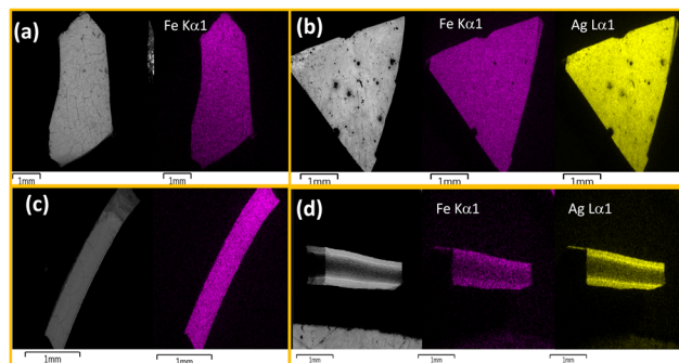
Fig. 5 SEM and SEM-EDS atomic mapping for the 1@chit surface (a), its transversal cut (c) and the 2@chit surface (b), its transversal cut (d). Iron atoms are shown in purple and silver one in yellow.
