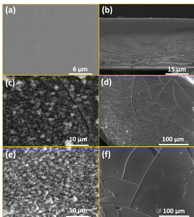
Fig. 4 SEM top film images of the chitosan film surface (a) and its transversal cut (b); (c) the 1@chit film surface (c) and its transversal cut (d); the 2@chit film surface (e) and its transversal cut (f).
