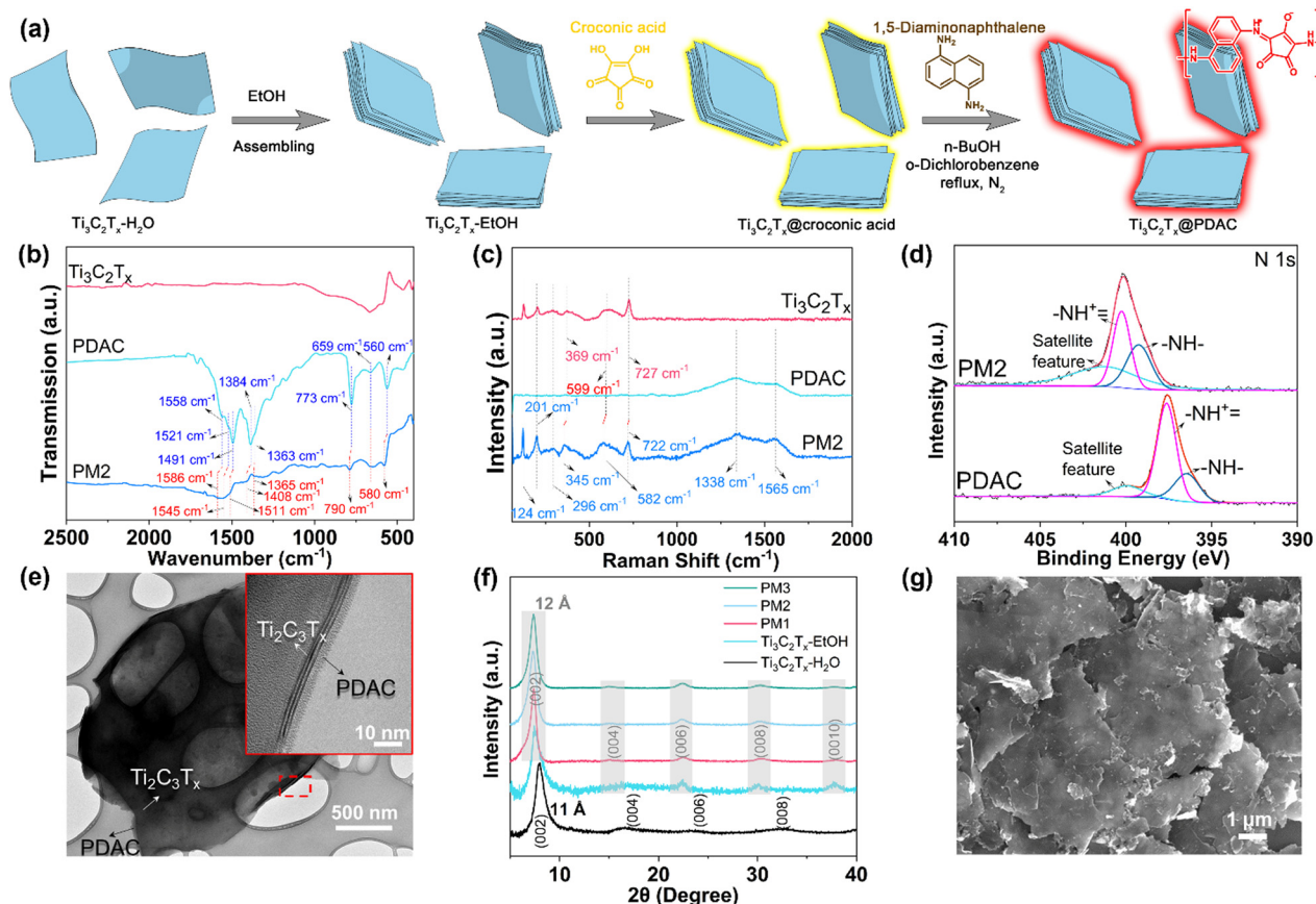
Fig. 1 Synthesis, chemical, and structural characterization of \text{Ti}_3\text{C}_2\text{T}_x @PDAC composites. (a) Schematic illustration of preparation of \text{Ti}_3\text{C}_2\text{T}_x @PDAC structure. (b) FTIR and (c) Raman spectra of \text{Ti}_3\text{C}_2\text{T}_x , PDAC, and PM2. (d) X-ray photoelectron spectra of the N 1s region of PM2 and PDAC. (e) TEM image of PM2, inset HRTEM image. (f) XRD patterns (baseline subtracted) of the composites and pristine \text{Ti}_3\text{C}_2\text{T}_x . (g) SEM image of PM2.
