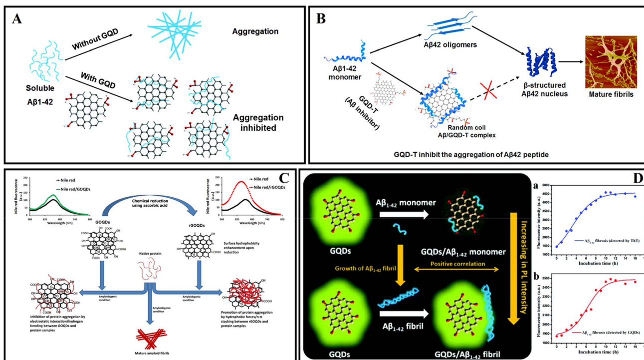
Fig. 12 (A) The GQDs used for inhibiting the aggregation of Aβ 42 peptides. 199 (B) GQD-T inhibits the aggregation of Aβ 42 peptides. 203 (C) GOQDs have the capacity to inhibit the fibrillation of protein. 208 (D) Proposed mechanism for the different fluorescence behaviors of GQDs on Aβ 42 monomers and fibrils. 209
