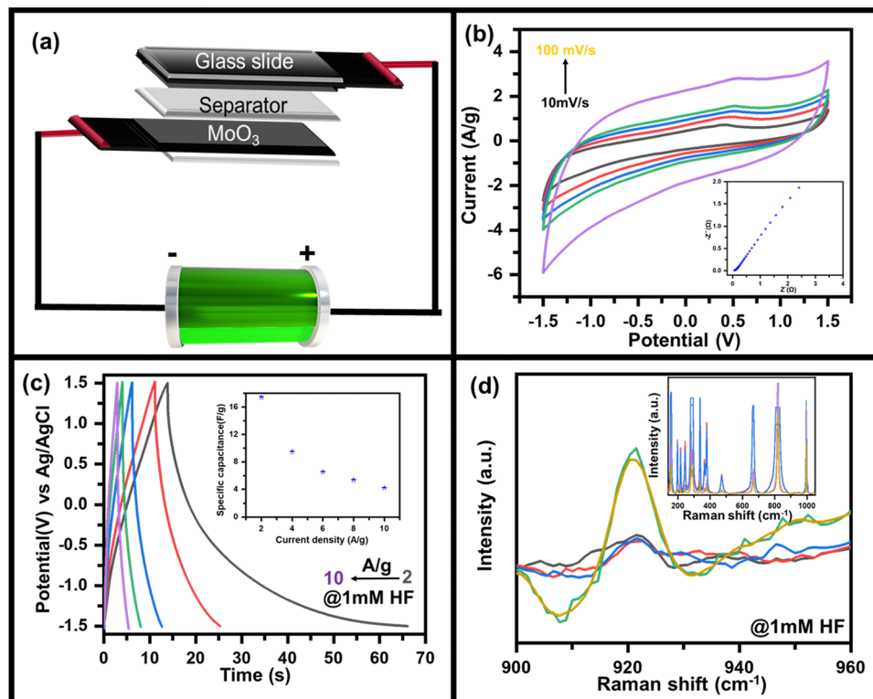
Fig. 4 (a) Schematic diagram of as-fabricated MoO 3 //AC supercapacitor device, (b) CV curves measured at scan rates of 10 to 100 mV s -1 along with the corresponding EIS plot (ESI†), (c) GCD plots at 2 A g -1 to 10 A g -1 along with variation of specific capacitance as a function of current density (inset) and (d) in situ Raman spectra of asymmetric supercapacitor device during the charging and discharging process.
