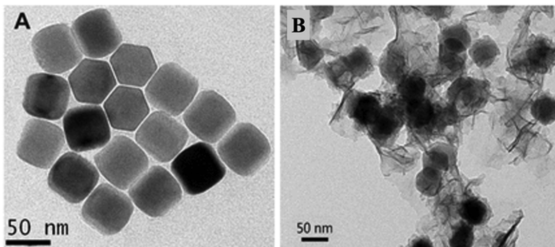
Fig. 13 TEM images (A) of OA-capped \text{NaYF}_4:\text{Yb,Tm}@ \text{NaYF}_4 core shell UCNPs, and (B) of \text{MnO}_2 NS-modified \text{NaYF}_4:\text{Yb,Tm}@ \text{NaYF}_4 UCNPs assemblies. 67 Copyright©2015, American Chemical Society.
