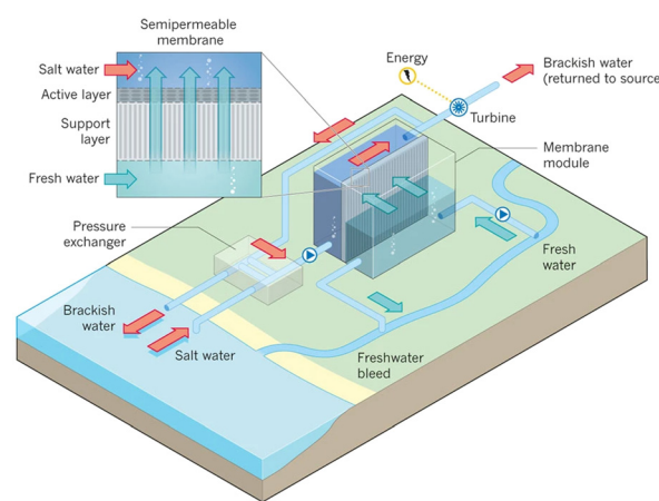
Fig. 10 Schematic illustration of the working principle of PRO systems. Feed solution and draw solution are injected continuously into water compartments which are separated by semipermeable membranes. Driven by effective osmotic force, water flux flows across the membrane from freshwater compartment towards saltwater compartment, resulting in a concentration decrease and a flow rate increase in draw solution compartment. The pressurized water flux is then split into two fluid streams: one fluid stream is used for electricity generation by driving an installed turbine, while the other stream returns to a pressure exchanger to maintain the pressure of draw solution (figures and captions reproduced from ref. 80 with permission from Springer Nature, copyright 2012).
