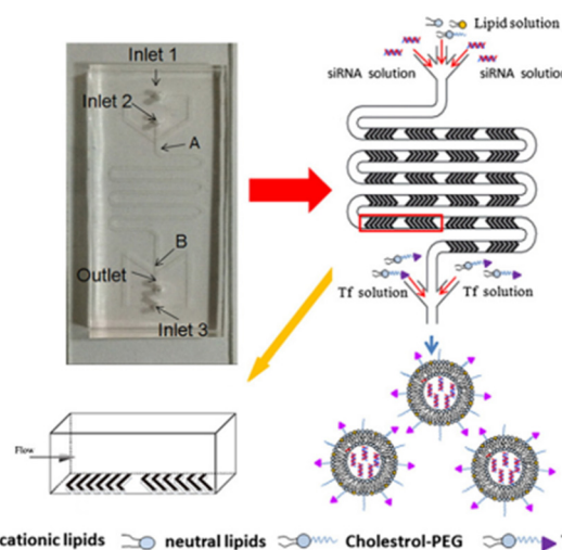
Fig. 7 Schematic representation of Tf-LNP fabrication using the staggered herringbone micromixer. Reprinted with permission from ref. 99. Copyright 2016. Elsevier.
