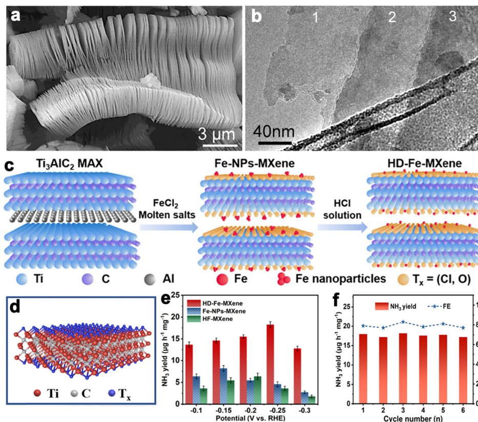
Fig. 9 (a and b) SEM and TEM images of Ti_3AlC_2 layers (reproduced from ref. 179 with permission from the American Chemical Society, copyright 2012). 179 (c) Schematic synthesis process of HD-Fe-MXene. (d) Crystal structure of Ti_3C_2T_x MXene. (e) NH_3 yields for the samples at different potentials. (f) NH_3 yields of HD-Fe-MXene and FEs during six cycles at -0.25 V versus RHE in 0.1 M Na_2SO_4 (reproduced from ref. 180 with permission from Wiley, copyright 2022). 180
