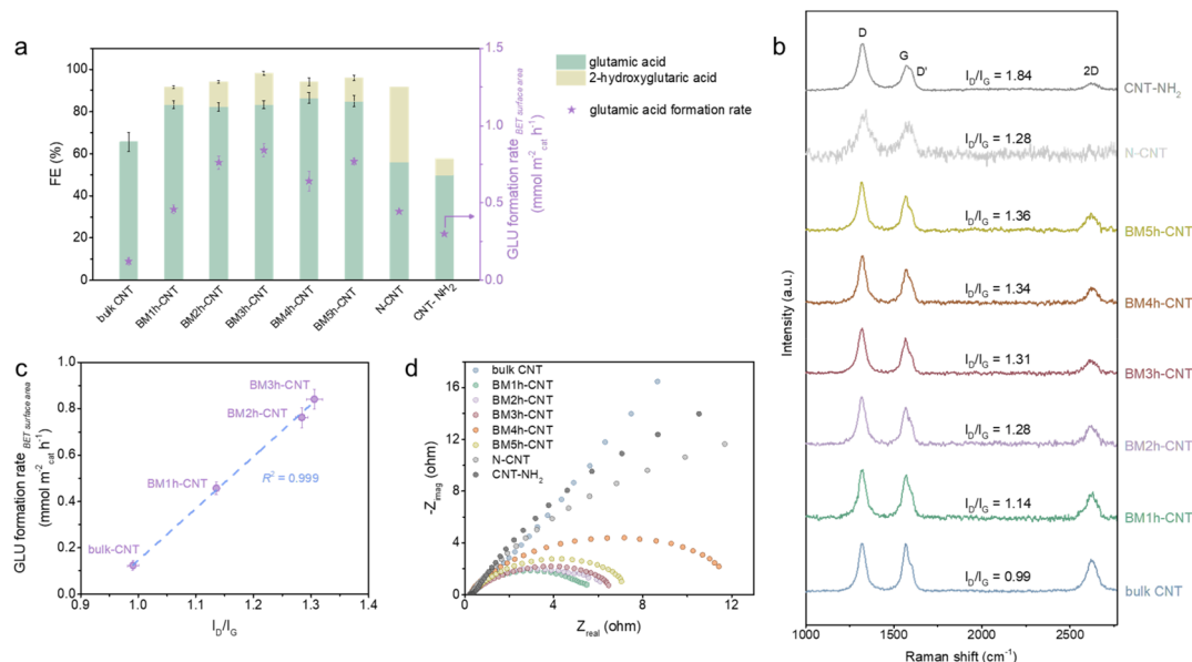
Fig. 4 Correlation of glutamic acid synthesis activity and CNT structure. (a) FE and GLU formation rate BET surface area of room-temperature electro-synthesis of 100 mM 2-ketoglutaric acid and 3 M NH 3 (pH 10) at -0.39 V vs. RHE for 1 h with different CNT materials. (b) Raman spectra of various CNT materials. (c) Correlation of CNT defective level I_D/I_G and surface area normalised glutamic acid formation rate. (d) Electrochemical Impedance Spectra (EIS) Nyquist plots of various CNT materials at -0.29 V vs. RHE in 100 mM 2-ketoglutaric acid and 3 M NH 3 /NH 4 + buffer (pH 10) solutions. The error bars denote the standard deviation of data from three independent experiments.
