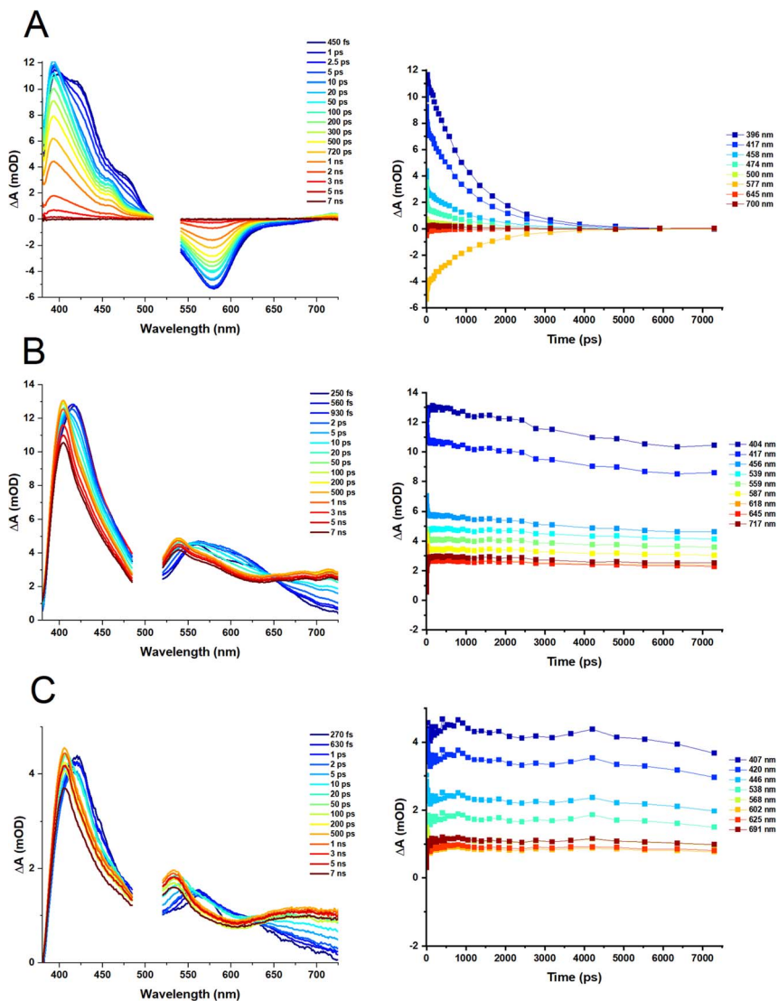
Fig. 6 Fs-TA of (A) D1, (B) D2 and (C) D3 in DCM. Fs-TA for D2 and D3 was recorded following excitation at 500 nm (2 mW, OD@500\text{ nm} = 0.38 (D2) and 0.2 (D3)). Fs-TA for D1 was recorded following photoexcitation at 525 nm (2 mW, OD@525\text{ nm} = 0.2 ). The spectra were collected with the pump set to magic angle ( 54.7^\circ ) with respect to the probe. The spectra have been cropped around the pump excitation wavelength to remove the pump scatter. The time delay between the pump and probe for each spectrum is shown in the legend. Kinetics for each complex are shown corresponding wavelength is shown in the legend.
