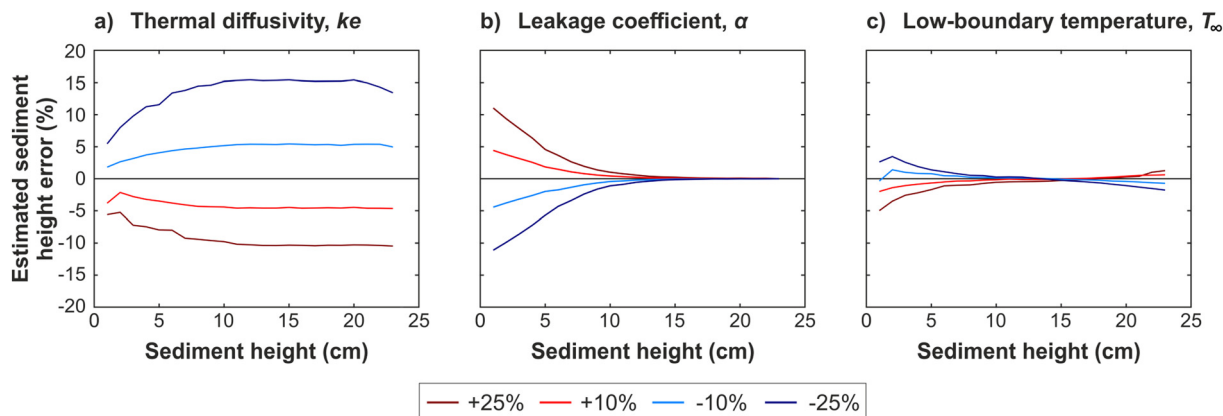
Fig. 9 Relative error of the sediment height estimations due to the change of thermal properties (a) and low-boundary conditions (b and c).
