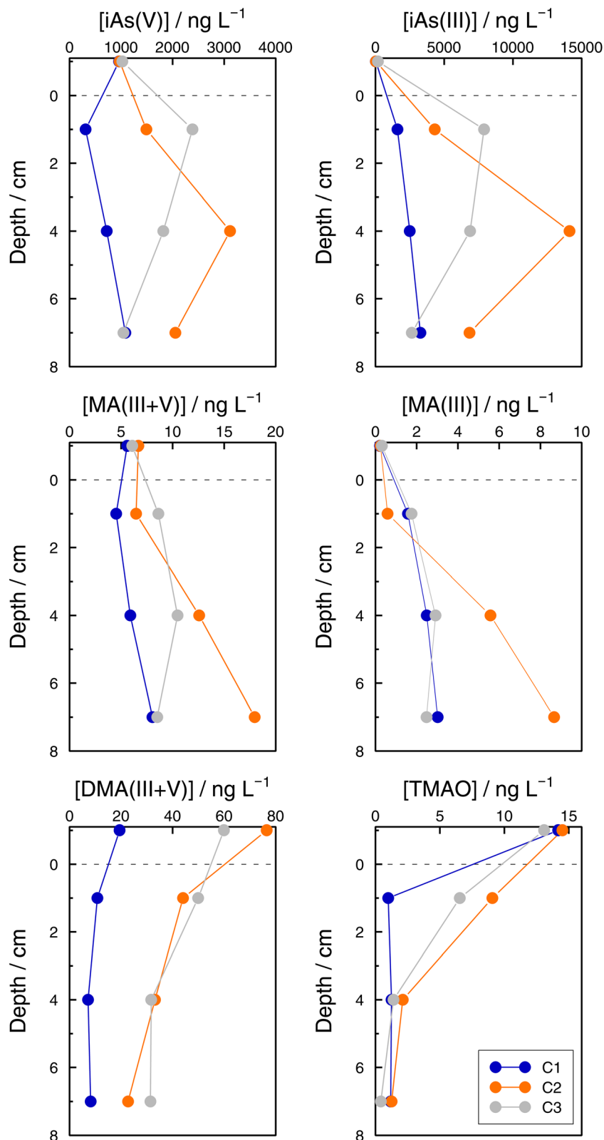
Fig. 8 Concentrations of total dissolved arsenic ( As_{tot,diss} ), iAs(V) , iAs(III) , MA(III + V) , DMA(III + V) , and TMAO concentrations in sediment pore waters and the overlying supernatant water in three cores (C1 (blue), C2 (orange), and C3 (grey)) in the Petit Lac, 12 July 2021.
