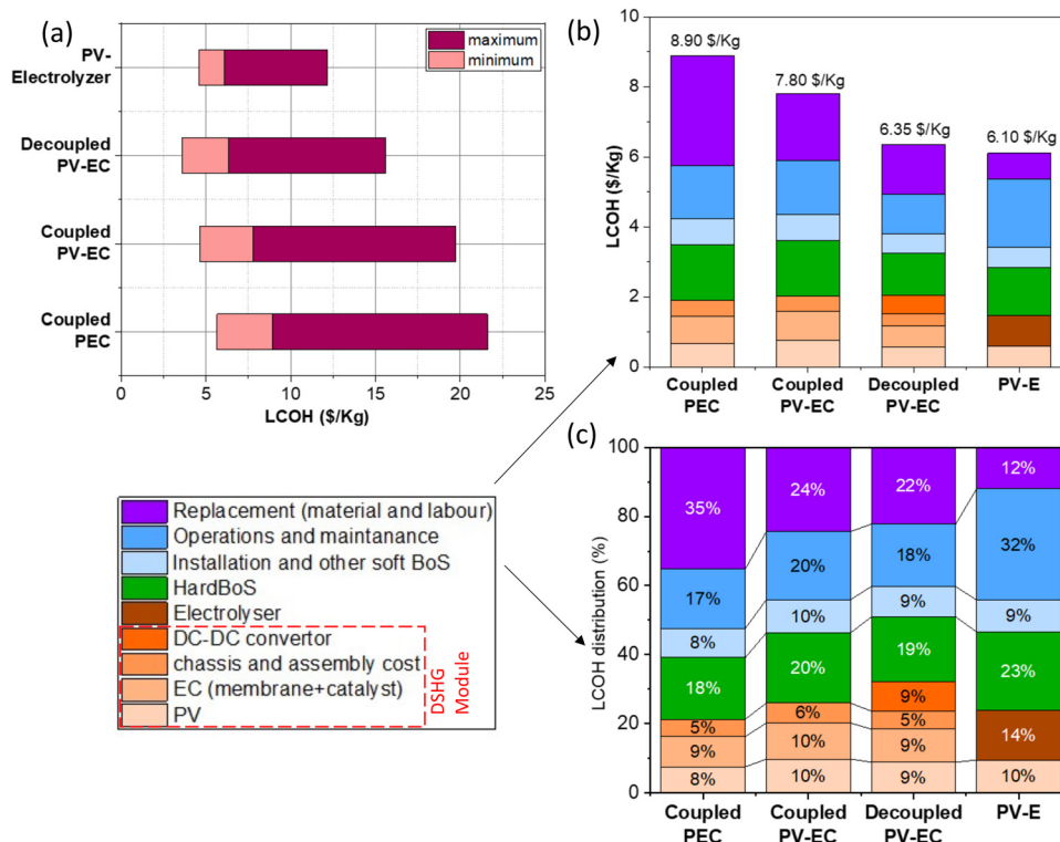
Fig. 2 (a) Range of levelized cost of hydrogen (LCOH) for all direct solar hydrogen generation (DSHG) systems and PV–Electrolyzer for range of component costs, given in Table S3 and S4 in the ESI†, (b) LCOH for all DSHG systems and PV–Electrolyzer for baseline costs with cost breakdown and (c) percentage contribution of different components, divided into module cost (PV, EC, chassis and assembly, dc–dc convertor, electrolyser), hard BoS, soft BoS, operations and maintenance (O&M) and replacement (material and labour) costs.
