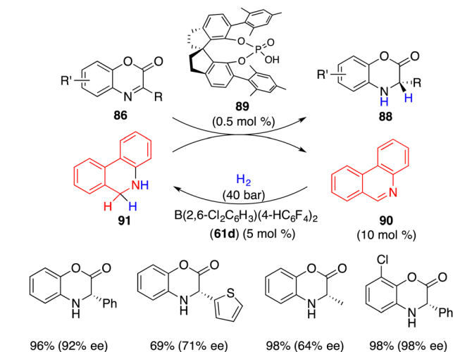
Scheme 50 Asymmetric transfer hydrogenation of benzoxazinones.
