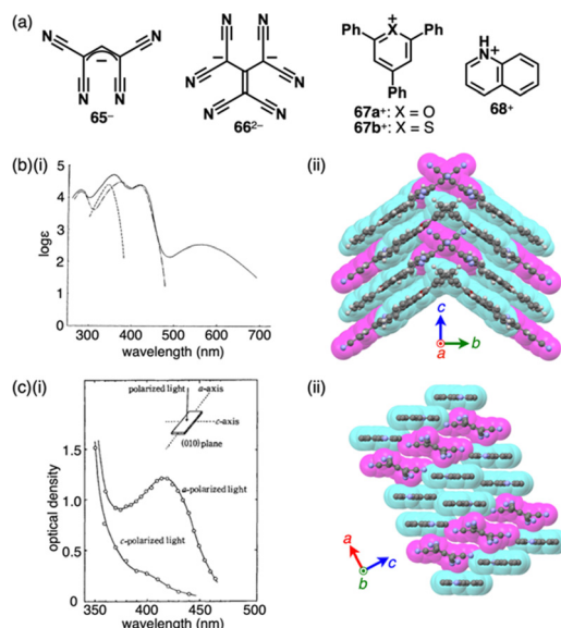
Fig. 39 Monomethine-based cyanocarbon anions and the counterions, (b) (i) UV/vis absorption spectra of 67a^+-65^- (solid line), 67a^+-\text{ClO}_4^- (chain line) and \text{Na}^+-65^- (dashed line) in \text{CHCl}_3 (redrawn from ref. 88a. Copyright 1970 CSJ) and (ii) single-crystal X-ray structure of 67a^+-65^- and (c) (i) polarized absorption spectra of 268^+-66^{2-} along with the direction of the long and short axes (redrawn from ref. 89a. Copyright 1969 CSJ) and (ii) single-crystal X-ray structure of 268^+-66^{2-} . The long axes of single crystals of 67a^+-65^- and 268^+-66^{2-} corresponded to the c and a axes in (ii), respectively. The crystal structures are redrawn from cif files: 1240563 and 1245498.
