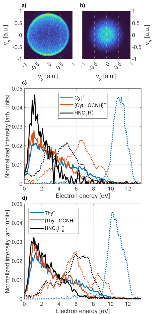
Fig. 7 VMIs of electrons in coincidence with Cyt + recorded for (a) direct photoionization of effusive Cyt ( h\nu = 20.6 eV) and (b) Penning ionization of Cyt in HNDs ( h\nu = 21.6 eV). Panels (c) and (d) show PIES ( h\nu = 21.6 eV) of HND-doped Cyt and Thy, respectively, for the three main electron-ion coincidence channels (solid lines). The dotted lines show the corresponding electron spectra of effusive Cyt and Thy ( h\nu = 20.6 eV).
